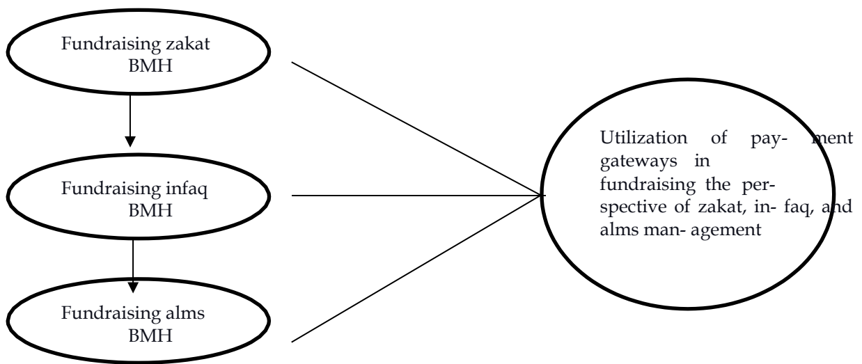
Figure 1. Framework
