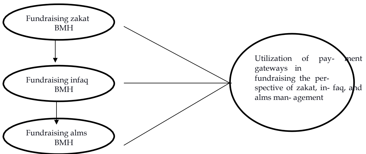
Figure 1. Framework
