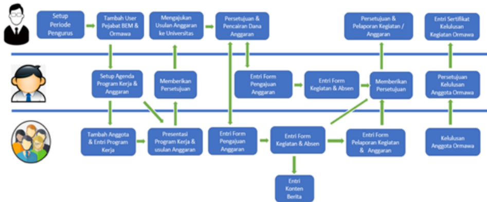
Gambar 3. Activity Diagram
