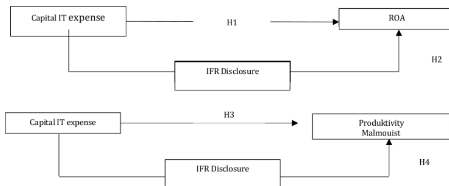
Figure 1: Research Design
