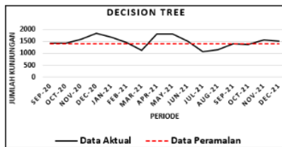
Gambar 6. Hasil Model Peramalan Decision Tree
