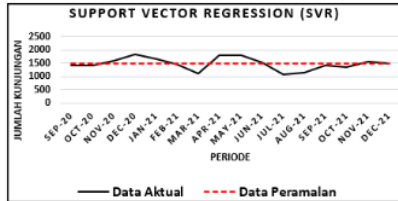
Gambar 4. Hasil Model Peramalan SVR
