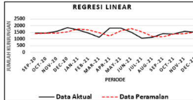
Gambar 8. Hasil Model Peramalan Regresi Linear
